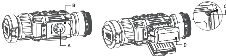
FIGURE 2-1. BATTERY INSTALLATION
