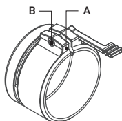
FIGURE 2-7. FRONT ADAPTER LEVER ADJUSTMENT
