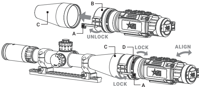
FIGURE 2-6. CLIP-ON INSTALLATION
