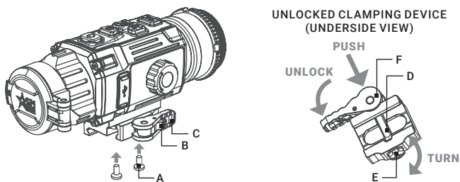
FIGURE 2-8. MOUNT
