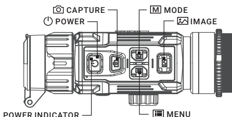
FIGURE 2-2. CONTROL BUTTONS
