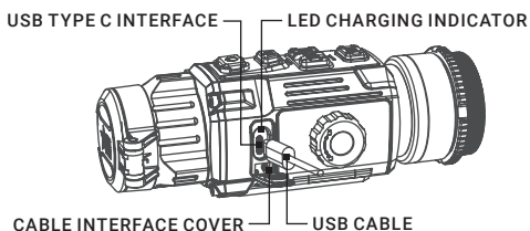
FIGURE 2-4. CABLE INTERFACE
