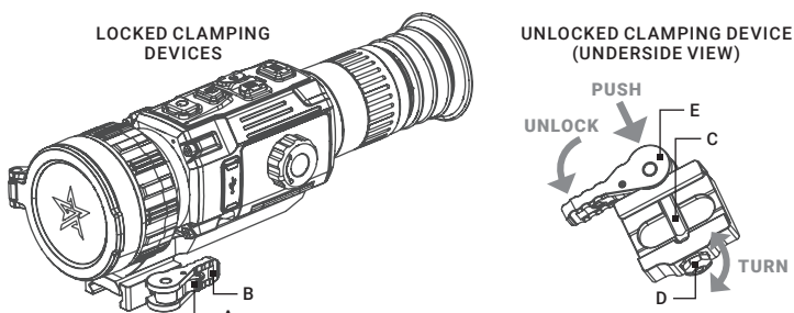
FIGURE 2-5. MOUNT
