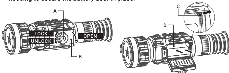
FIGURE 2-1. BATTERY INSTALLATION
