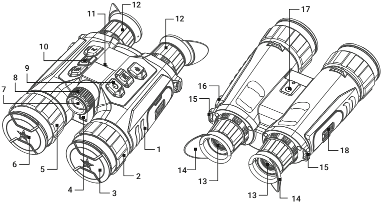
FIGURE 1-2. MAIN PARTS
