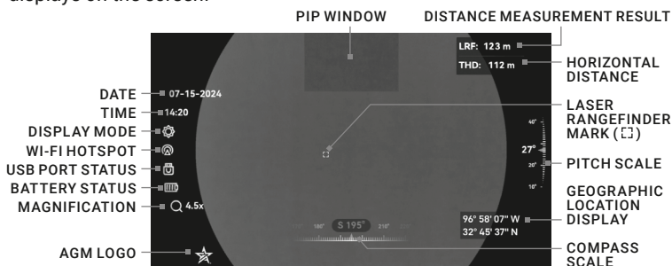
FIGURE 2-6. ON-SCREEN DISPLAY
