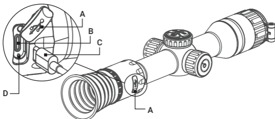
FIGURE 2-1. USB INTERFACE
