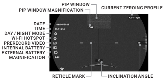
FIGURE 2-4. ON-SCREEN DISPLAY
