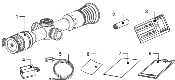
FIGURE 1-2. STANDARD COMPONENTS
