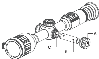
FIGURE 2-2. ADDITIONAL BATTERY INSTALLATION
