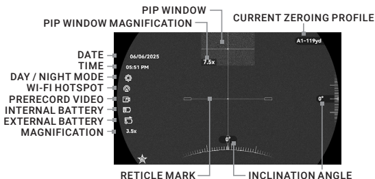
FIGURE 2-4. ON-SCREEN DISPLAY
