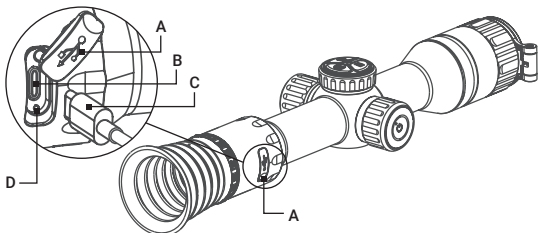
FIGURE 2-1. USB INTERFACE
