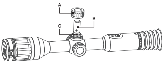
FIGURE 2-2. CR123A BATTERY INSTALLATION
