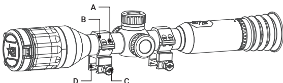
FIGURE 2-5. INSTALLATION WITH SCOPE RINGS
