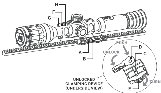
FIGURE 2-6. INSTALLATION WITH QUICK RELEASE MOUNT
