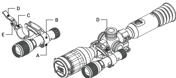
FIGURE 2-7. IR ILLUMINATOR INSTALLATION
