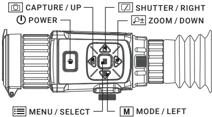
FIGURE 2-2. CONTROL BUTTONS
