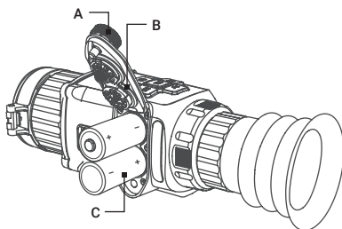
FIGURE 2-1. BATTERY INSTALLATION
