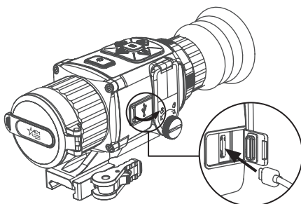
FIGURE 2-4. CABLE INTERFACE
