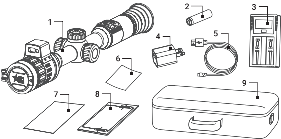
FIGURE 1-2. STANDARD COMPONENTS
