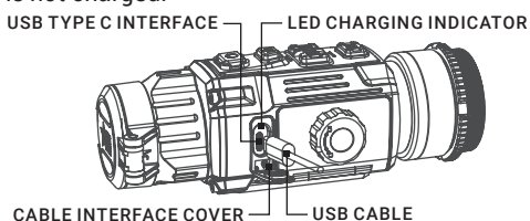
FIGURE 2-4. CABLE INTERFACE
