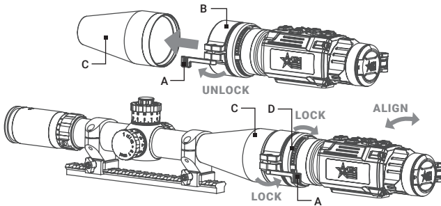
FIGURE 2-6. CLIP-ON INSTALLATION
