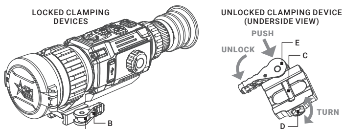
FIGURE 2-5. MOUNT
