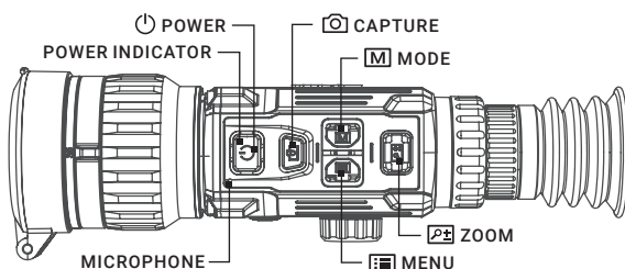
FIGURE 2-2. CONTROL BUTTONS
