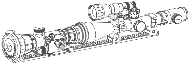
FIGURE 2-6. SIOUX850 IR ILLUMINATOR INSTALLATION
