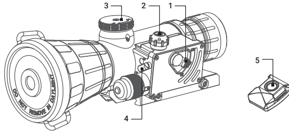
FIGURE 2-8. COMANCHE-40ER CONTROLS AND INDICATOR
