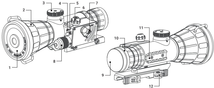
FIGURE 1-1. COMANCHE-40ER NIGHT VISION CLIP-ON MAIN PART
