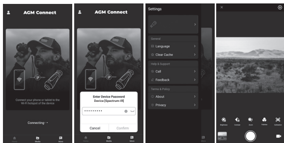
FIGURE 2-14. CLIENT SOFTWARE
