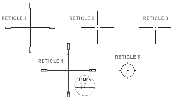
FIGURE 2-11. RETICLE PATTERNS
