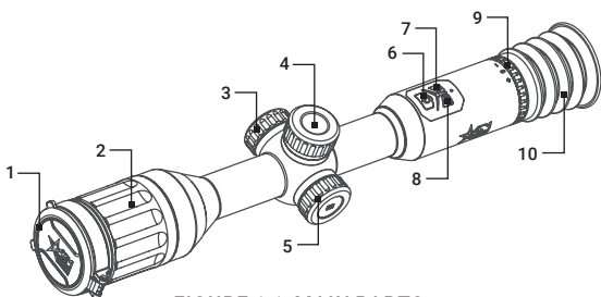
FIGURE 1-1. MAIN PARTS
