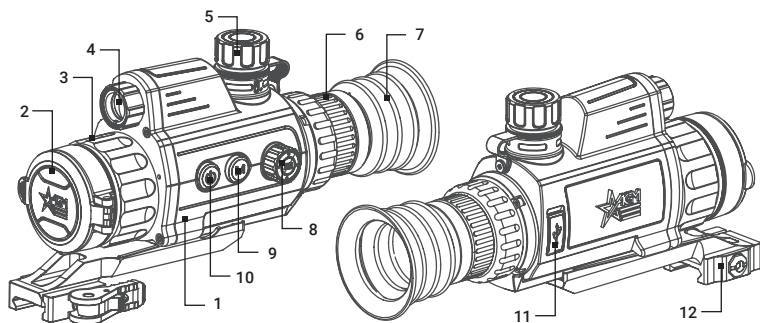
FIGURE 1-1. MAIN PARTS
