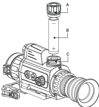
FIGURE 2-1. BATTERY INSTALLATION
