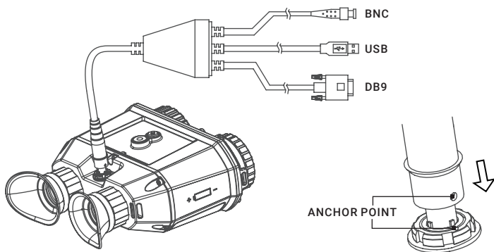
FIGURE 2-6. CABLE CONNECTION
