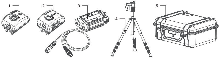
FIGURE 1-4. OPTIONAL EQUIPMENT
