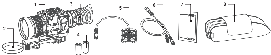
FIGURE 1-3. STANDARD COMPONENTS
