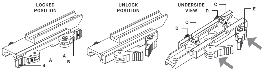
FIGURE 2-4. MOUNT
